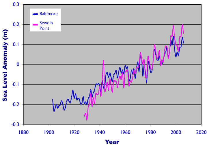
Figure 5. Long-term sea-level change at two locations in the Chesapeake Bay: Baltimore, MD (upper Bay) and Sewells Point, VA (lower Bay). Data are annual mean differences from the 1950 – 2000 average and were acquired from NOAA’s Center for Operational Oceanographic Products and Services.
