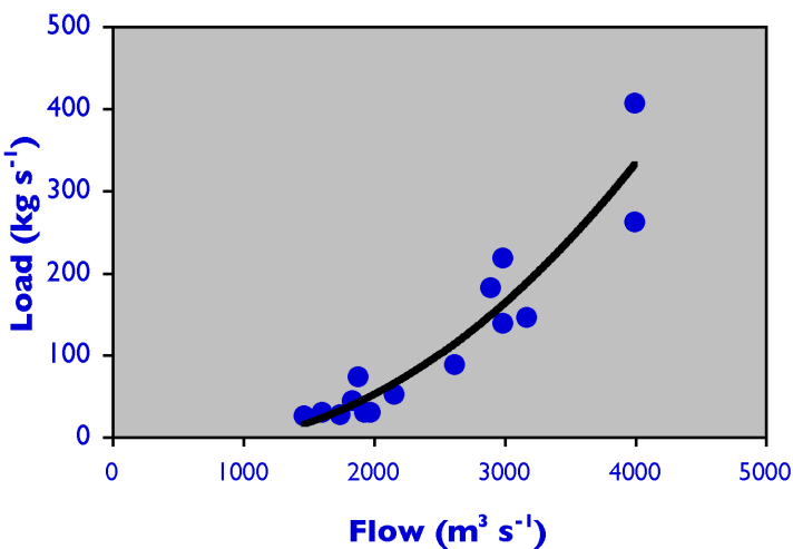
Figure 6. The relationship between annual sediment yield and total freshwater inflow to the Chesapeake Bay from 1990 to 2004. The curve is a least-squares parabolic fit ( r^2 = 0.88 ) with a forced zero intercept, y = 3 \times 10^{-5}x^2 - 0.0325x . The estimates come from the CBP website. The USGS computed the annual yields by summing the products of daily streamflow and riverine total suspended solids (TSS) concentrations. These TSS values are based on a statistical model calibrated with TSS observations from several monitoring stations. Langland et al. (2006, p. 13) offer details on data sources and methodology.
