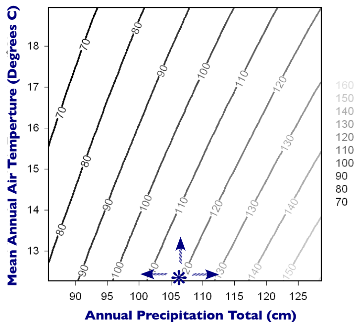
Figure 8. Annual nitrogen loading ( 10^3 \text{ kg yr}^{-1} ) in the Western Branch of the Patuxent River in Maryland as a function of annual precipitation and mean annual temperature (the * represents the historical average climate). The plot is based on a series of HSPF model simulations generated with the automated, iterative assessment capability in the BASINS Climate Assessment Tool (reprinted from Johnson and Kittle [2007]).
