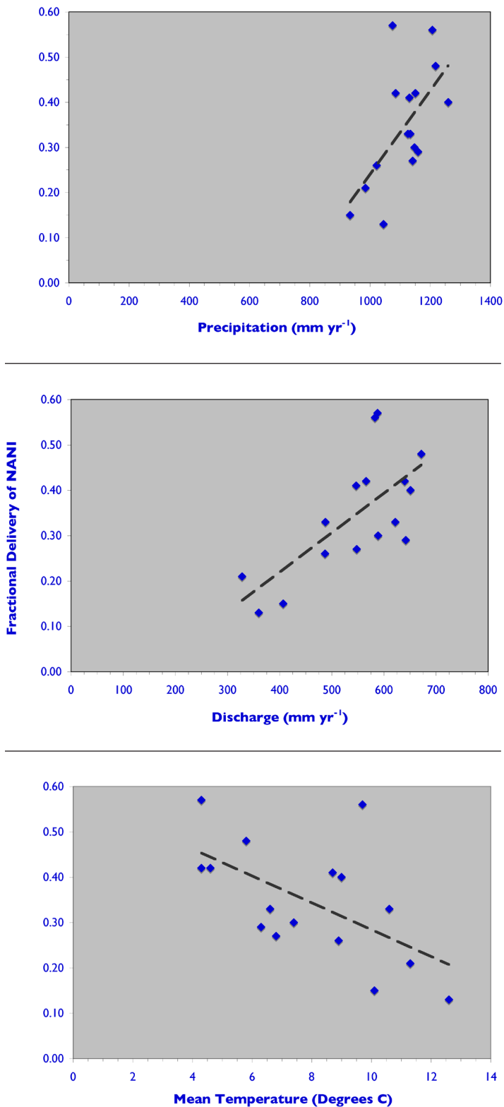
Figure 7. The fractional delivery of net anthropogenic nitrogen inputs (NANI) for 16 major watersheds in the northeastern United States plotted as a function of mean discharge, mean precipitation, and mean temperature. The relationships for discharge and precipitation are highly significant ( p = 0.003 and 0.0015 , respectively). The relationship for temperature is weaker ( p = 0.11 ) (taken from Howarth et al. [2006]).
