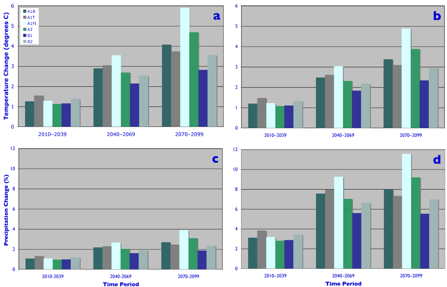
Figure 4. Projected change in the annual mean temperature (a and b) and precipitation (c and d) of the Chesapeake Bay watershed for six IPCC scenarios (see Figure 1) averaged over seven climate models (a and c) and the four highest ranked (b and d). From Najjar et al. [2008].
