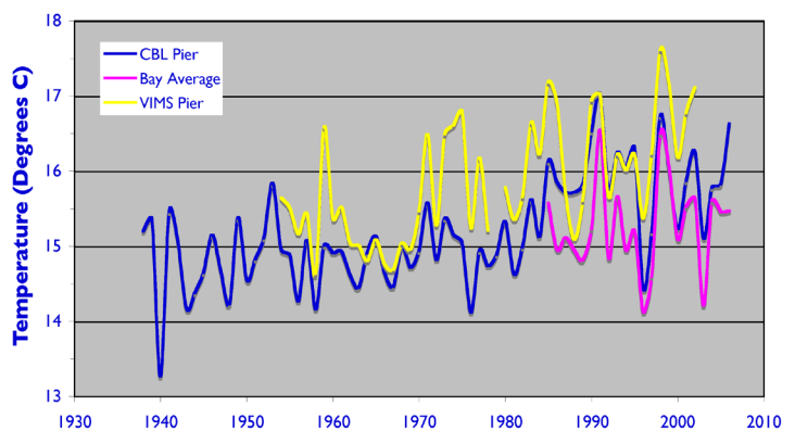
Figure 2. Annual average surface temperature from the mouth of the York River (VIMS pier), the mouth of the Patuxent River (CBL pier), and the average throughout the mainstem Bay (Bay average). The VIMS data come from Austin (2002) and the CBL data come from Secor and Wingate (2008). The VIMS data are part of the VIMS Scientific Data Archive, acquired from Gary Anderson at VIMS. David Jasinski, Chesapeake Bay Program Office, computed the Bay-average data using measurements from the Chesapeake Bay Water Quality Monitoring Program. Data were first averaged by month at each station, then by year, before taking the arithmetic mean of all stations.
